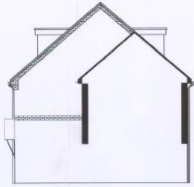
Existing West (side) elevation Scale 1:100
