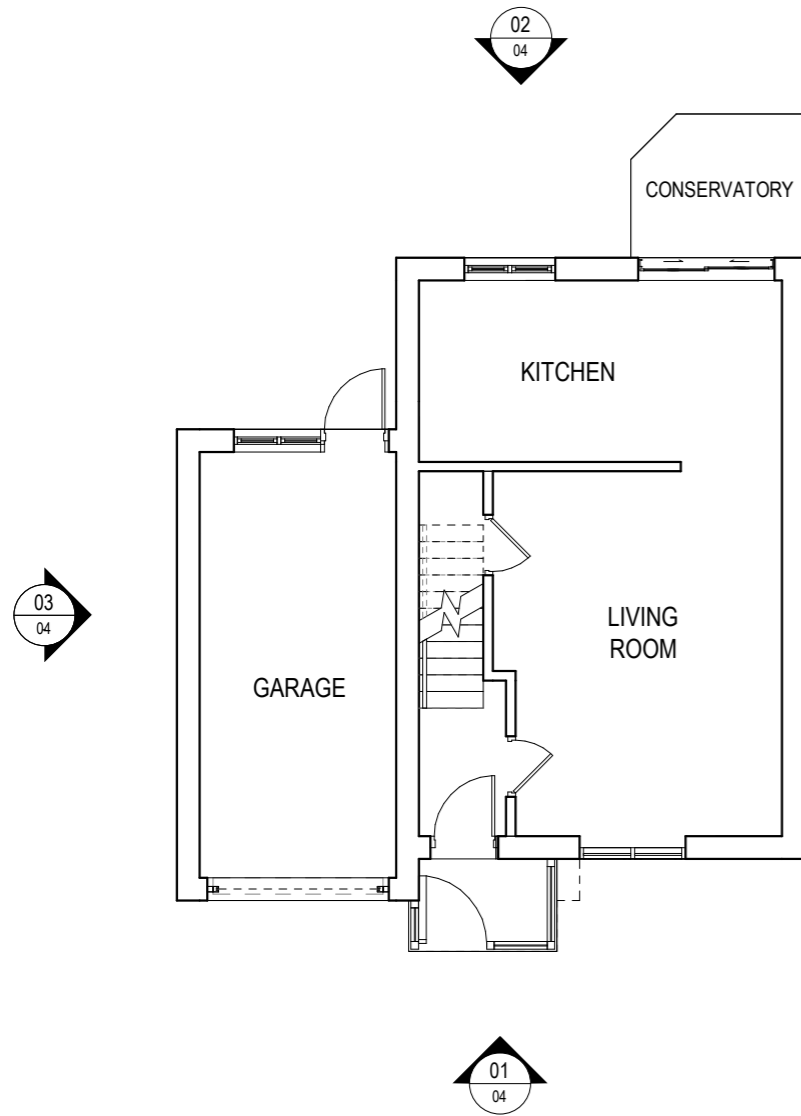
01 GROUND FLOOR SCALE 1 : 100
