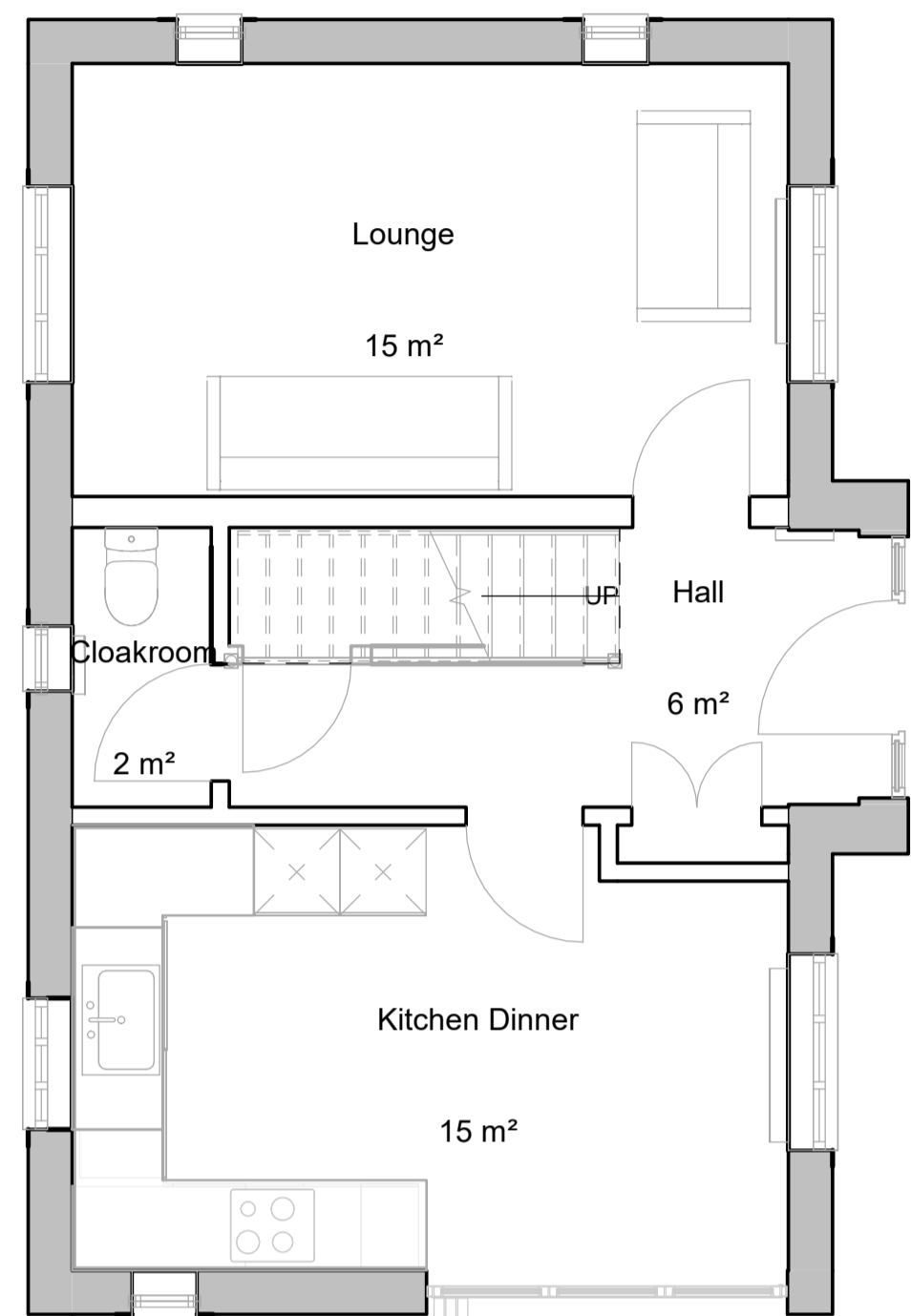
1 Ground Floor FFL 1:50
