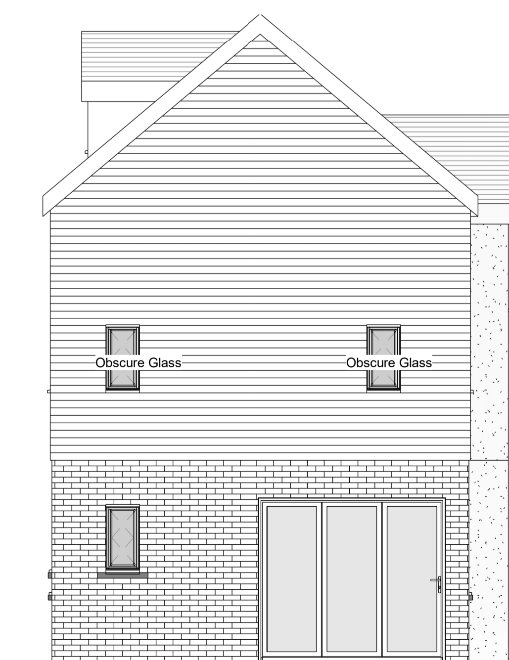
5 South 1:50
