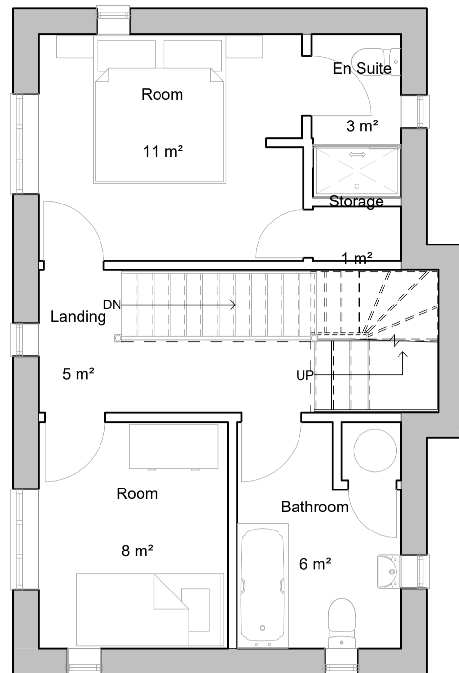
2 First Floor FFL 1:50
