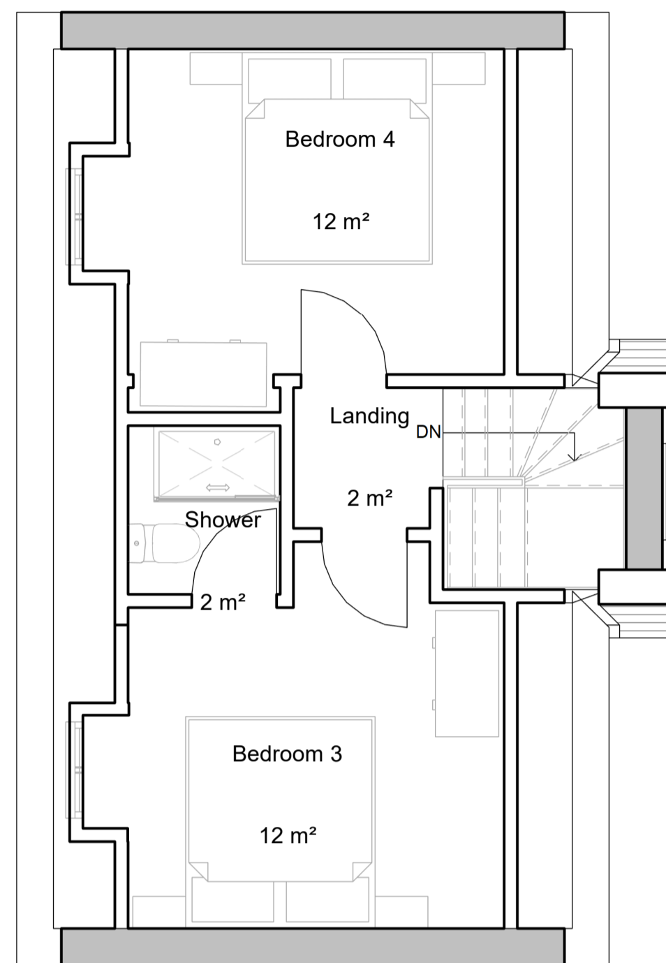
3 Upper floor FFL 1:50
