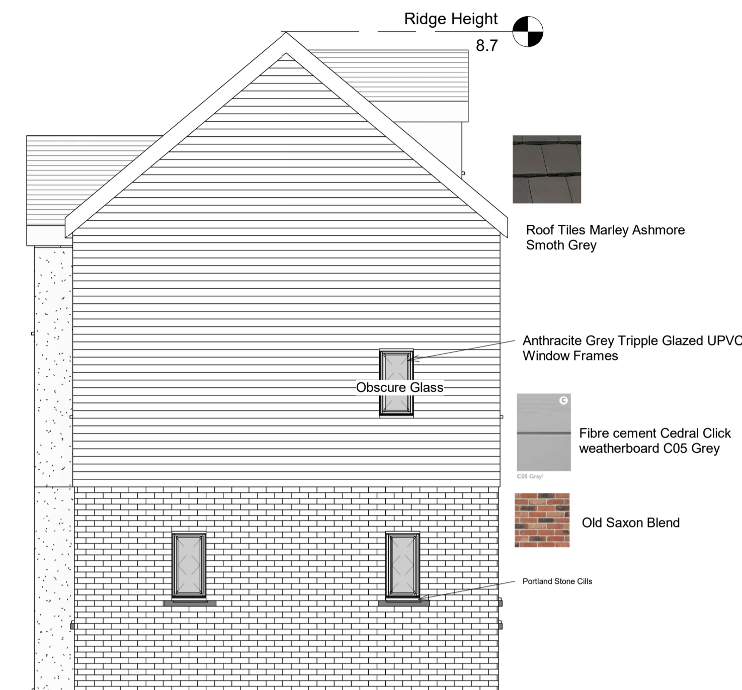
4 North 1:50
